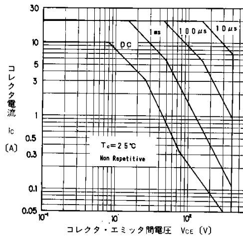
安全動作領域 Reverse Biased Safe Operating Area
