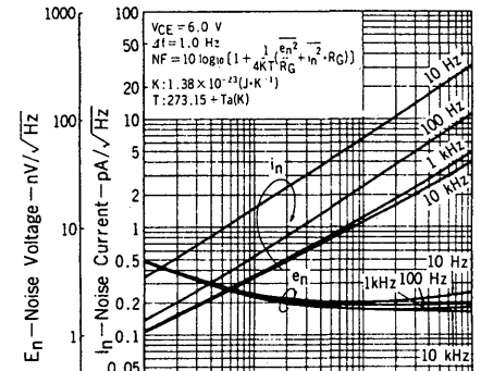
E_n AND I_n vs. COLLECTOR CURRENT
