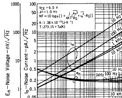
E_n AND I_n vs. COLLECTOR CURRENT
