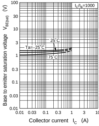
V_{BE(\text{sat})} - I_C
