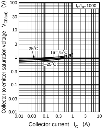
V_{CE(\text{sat})} - I_C
