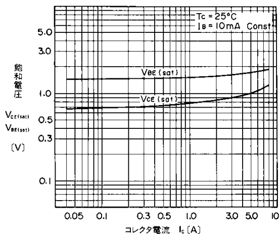
飽和電圧—コレクタ電流特性 Base and Collector Saturation Voltage
