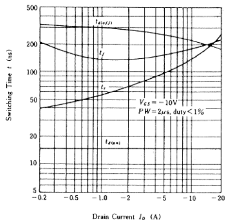
SWITCHING CHARACTERISTICS
