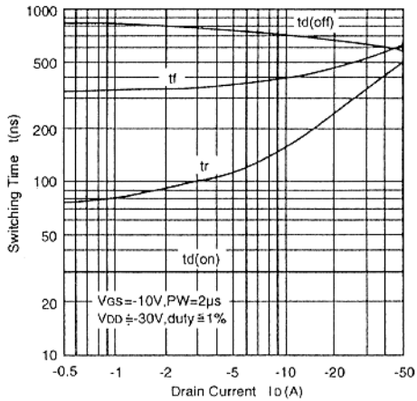
SWITCHING CHARACTERISTICS
