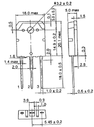
(TO-3P)
