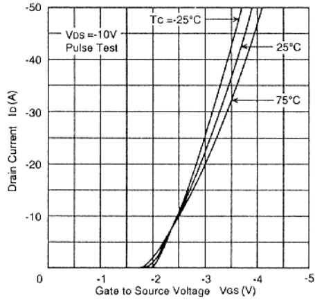
TYPICAL FORWARD TRANSFER CHARACTERISTICS
