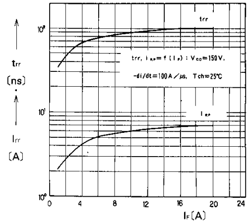
Reverse Recovery Characteristics
