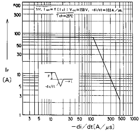
IF-di/dt Characteristics of Reverse Diode
