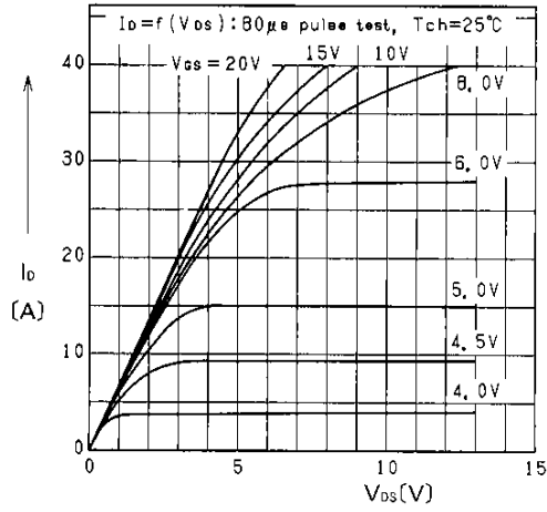
Typical Output Characteristics vs. V_{DS}
