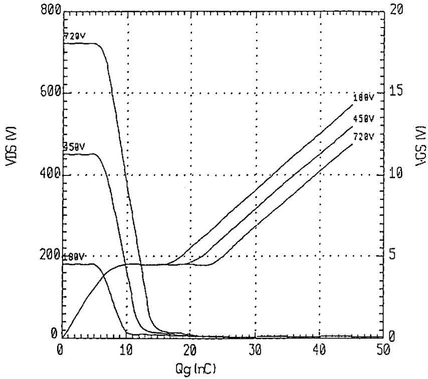
Typical gate charge characteristics V_{GS} = f(Q_g) : I_D = 4A
