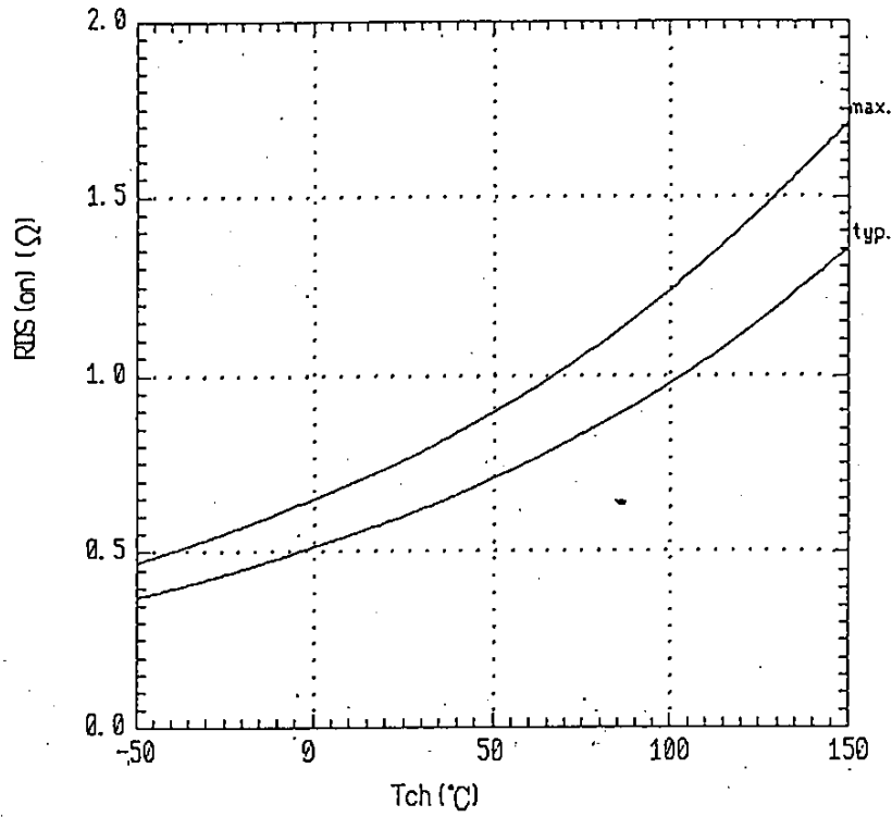
Drain-source on-state resistances R_{DS(on)} = f(T_{ch}) : I_D = 5A, V_{GS} = 10V
