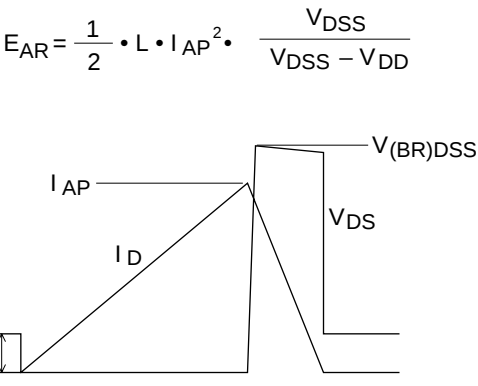
Avalanche Test Circuit and Waveform
