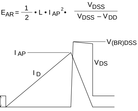
Avalanche Test Circuit and Waveform
