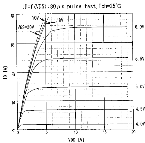
出力特性 Typical output characteristics
