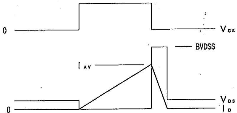
Fig.2 Operating waveforms
