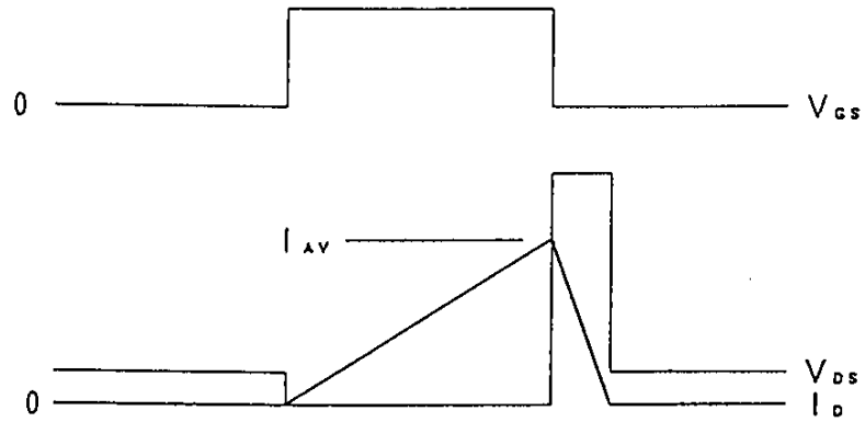
Fig.2 Operating waveforms
