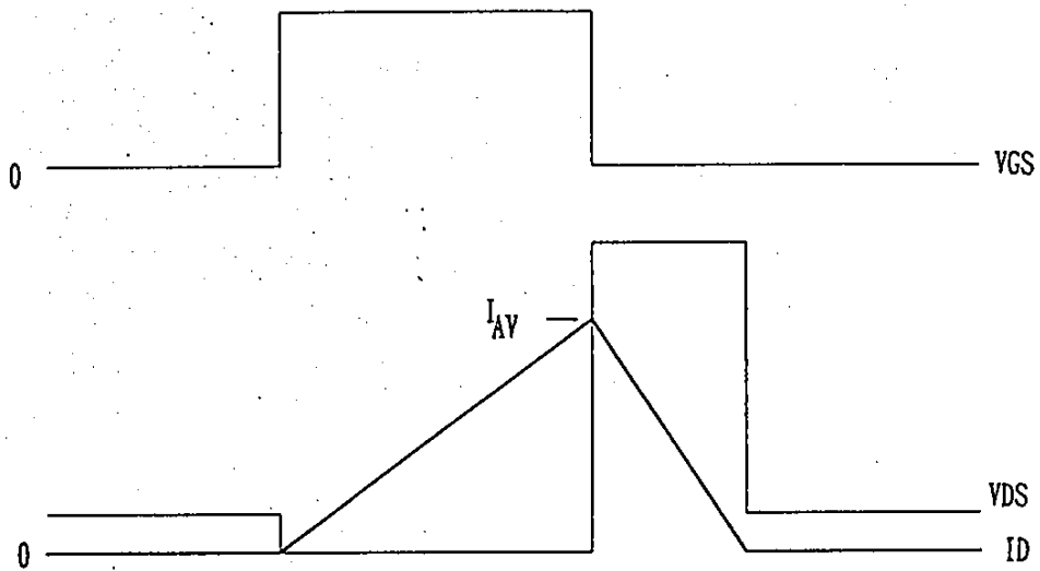
Fig.2 Operating waveforms
