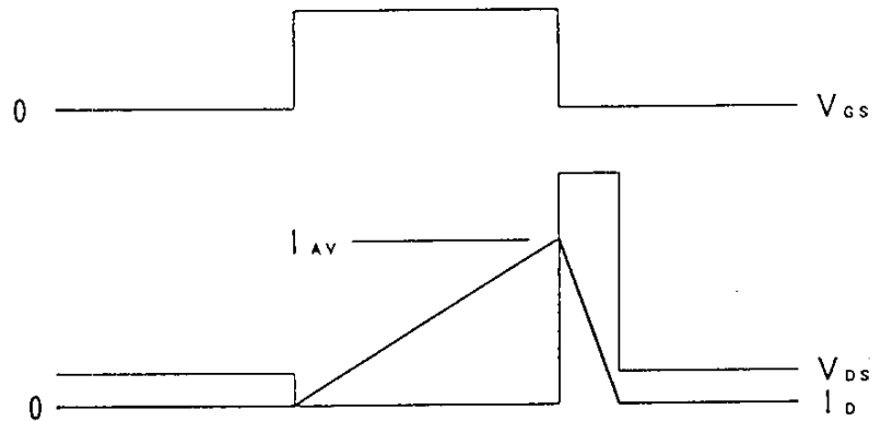
Fig.2 Operating waveforms
