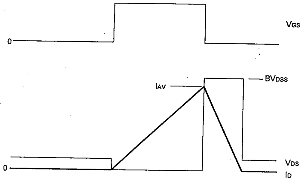
Fig.2 Operating waveforms
