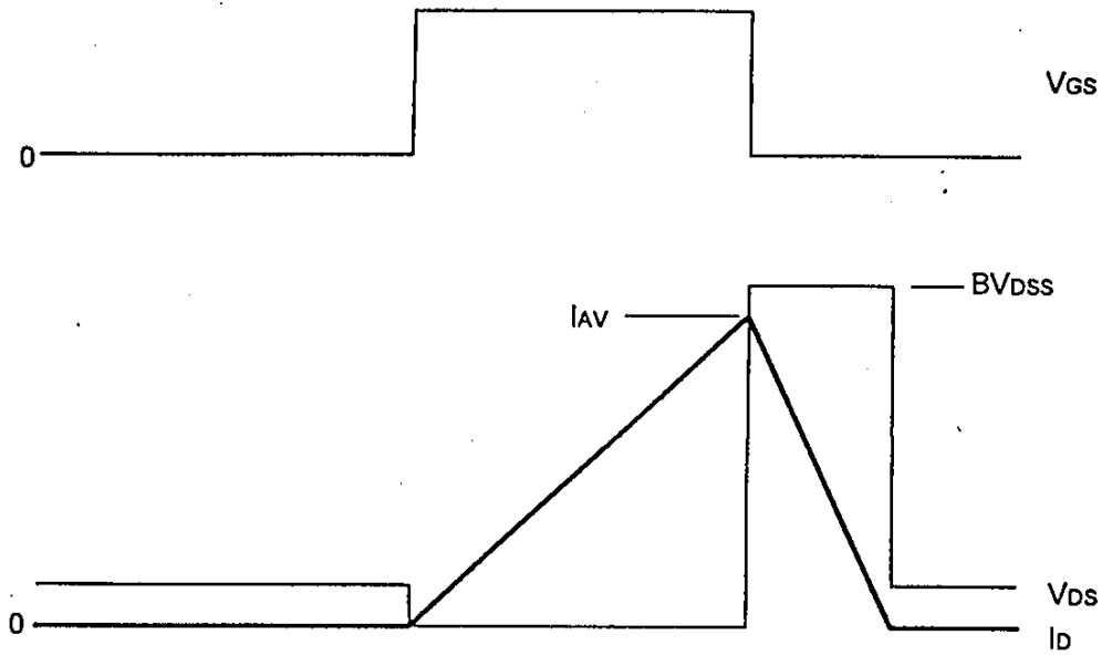
Fig.2 Operating waveforms
