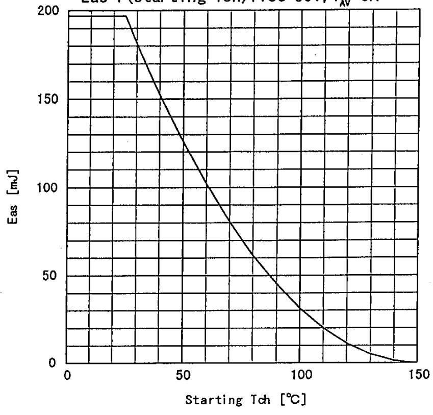
Avalanche energy derating E_{as}=f(\text{starting } T_{ch}): V_{cc}=50V, I_{AV}=6A
