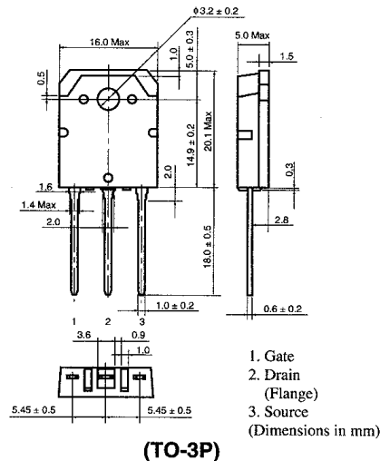
(TO-3P)
