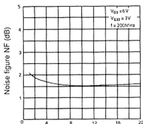
Noise figure vs. drain current
