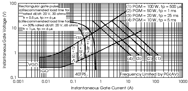
Fig. 8 - Gate Characteristics
