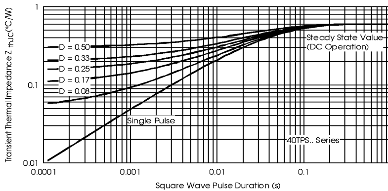
Fig. 9 - Thermal Impedance Z_{thjC} Characteristics
