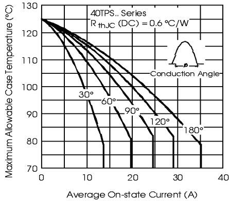
Fig. 1 - Current Rating Characteristics
