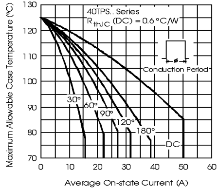
Fig. 2 - Current Rating Characteristics
