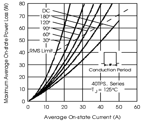
Fig. 4 - On-state Power Loss Characteristics
