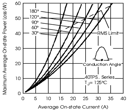
Fig. 3 - On-state Power Loss Characteristics
