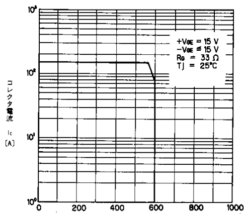
安全動作領域(逆バイアス) Reverse Biased Safe Operating Area
