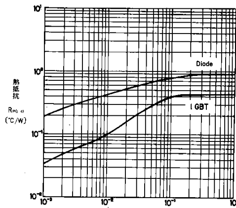
過渡熱抵抗 Transient Thermal Resistance
