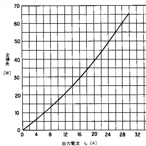
出力電流-全損失 Output Current-Total Loss
