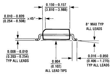
14-Lead (0.150" Wide) Molded Small Outline Integrated Circuit Package Number M14A
