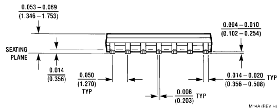
14-Lead (0.150" Wide) Molded Small Outline Integrated Circuit Package Number M14A
