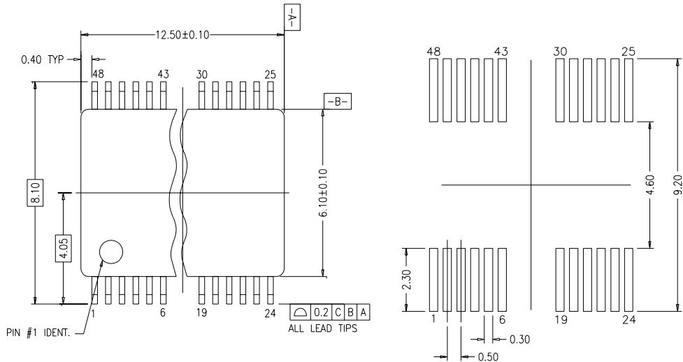
LAND PATTERN RECOMMENDATION
