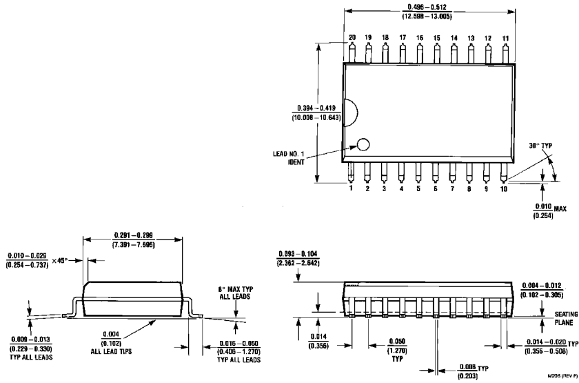
Order Number ADC10461CIWM NS Package Number M20B
