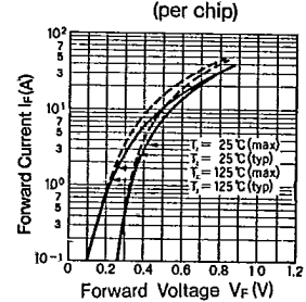
I_F - V_F Characteristics (per chip)
