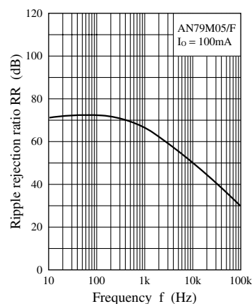
RR — f
