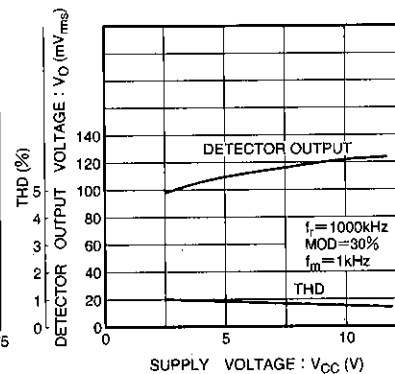
Fig. 42 AM THD and detector output voltage vs. supply voltage
