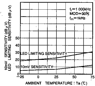
Fig. 45 AM 10mV sensitivity and LED limiting sensitivity vs. ambient temperature
