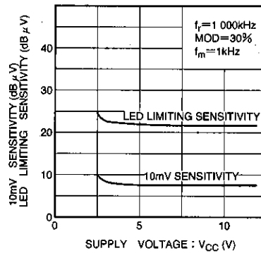
Fig. 44 AM 10mV sensitivity and LED limiting sensitivity vs. supply voltage
