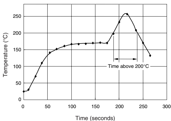
Reflow soldering profile (for reference only)
