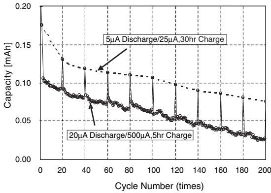
Charge-Discharge Cycle Characteristics (100% D.O.D)
