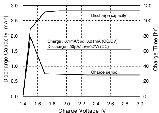
Charge voltage dependence of discharge capacity
