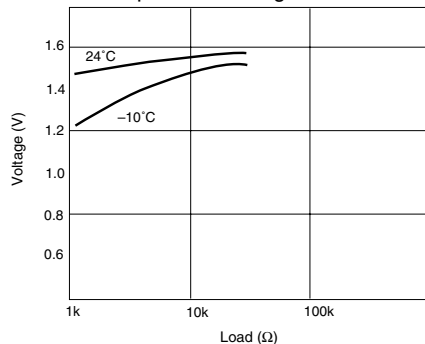
Load-temperature-voltage characteristics
