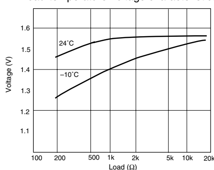
Load-temperature-voltage characteristics
