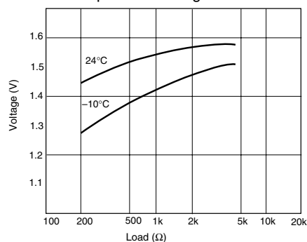
Load-temperature-voltage characteristics
