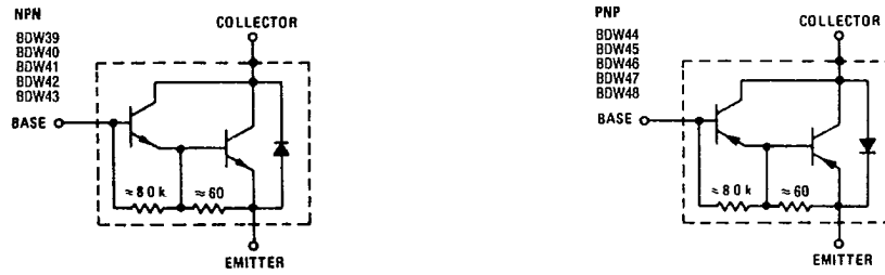
FIGURE 14 - DARLINGTON SCHEMATIC
