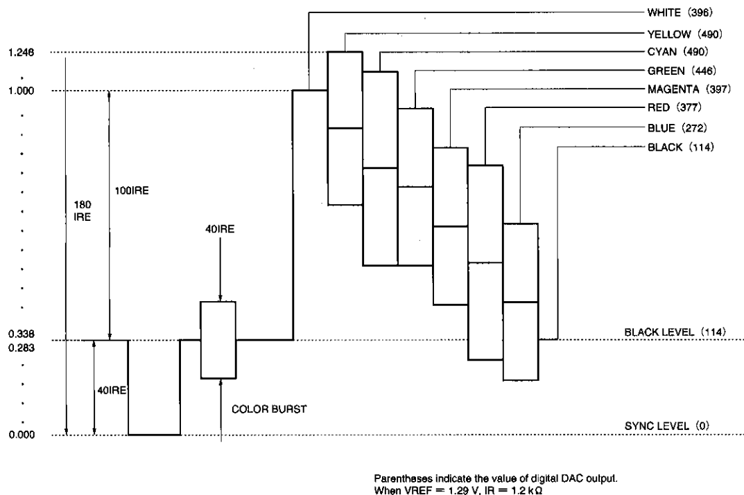
Fig. 3 NTSC V (composite) signal output level
