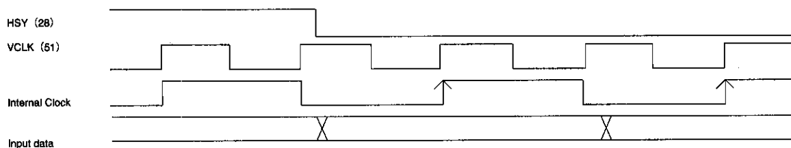
Fig. 2-3-1 Clock timing (CLKSW is at the low level)
