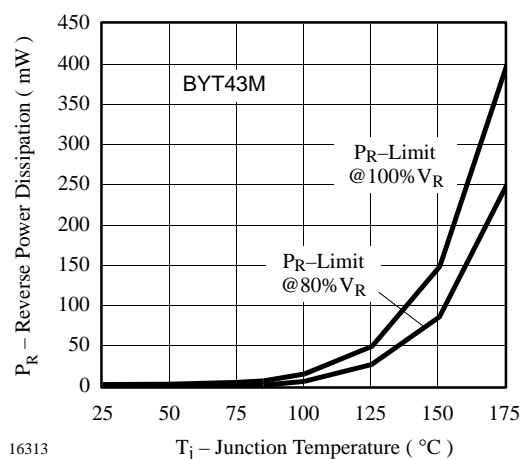
Figure 8. Max. Reverse Power Dissipation vs. Junction Temperature
