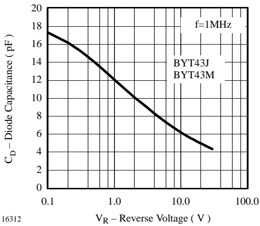
Figure 9. Diode Capacitance vs. Reverse Voltage
