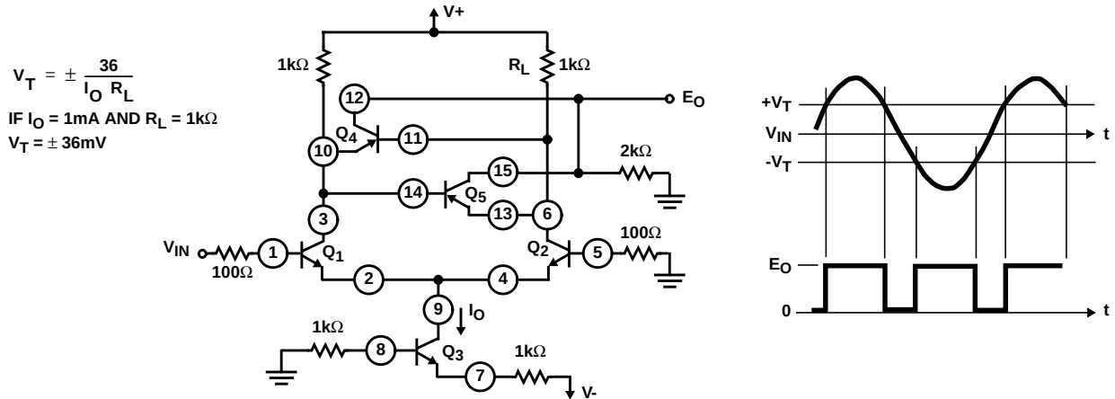
FIGURE 5. CA3096A SMALL-SIGNAL ZERO VOLTAGE DETECTOR HAVING NOISE IMMUNITY
