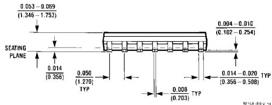
Molded Small Outline Package (M) Order Number CD4070BCM or CD4077BCM NS Package Number M14A
