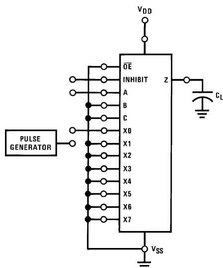
Input Connections for t_r , t_f , t_{PLH} , t_{PLL}
