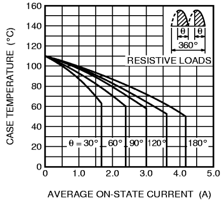
ALLOWABLE CASE TEMPERATURE VS. AVERAGE ON-STATE CURRENT (SINGLE-PHASE FULL WAVE)
