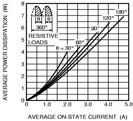
MAXIMUM AVERAGE POWER DISSIPATION (SINGLE-PHASE FULL WAVE)
