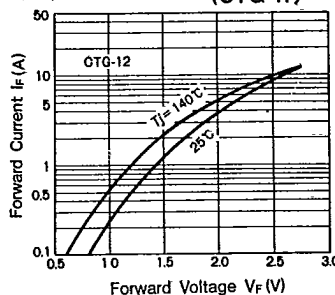
I F -V F Characteristics (CTG-12)
