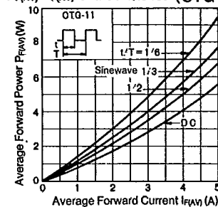
P F(AV) -I F(AV) Characteristics (CTG-11)
