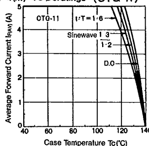
I F(AV) -T c Deratings (CTG-11)
