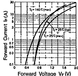
I F - V F Characteristics (Typical Value) CTL-22S
