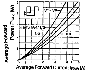
P F(AV) - I F(AV) Characteristics
