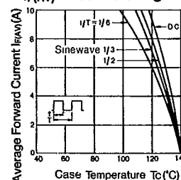
I F(AV) - T c Derating
