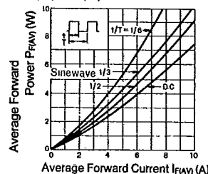
P F(AV) - I F(AV) Characteristics
