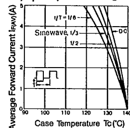
I F(AV) - T pin Derating
