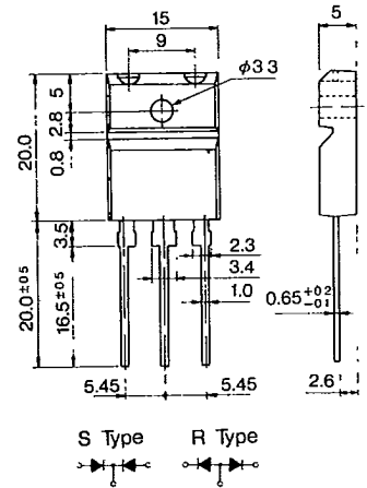
Outline Drawing ④⑥
