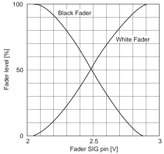
Y fader control characteristics
