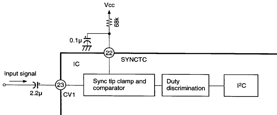
Fig. 1. Sync discrimination circuit block diagram
