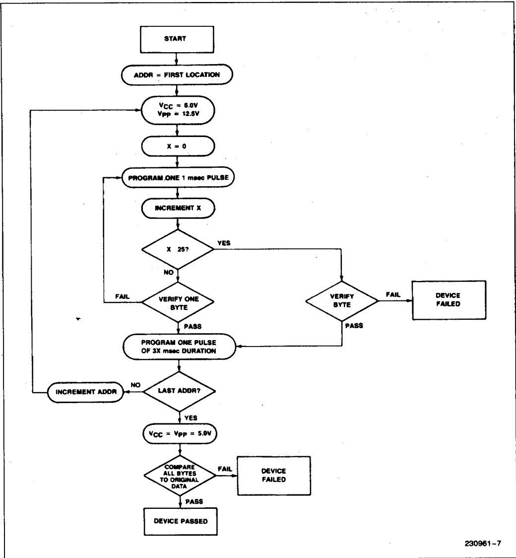
Figure 3. M27256 intelligent Programming™ Flowchart
