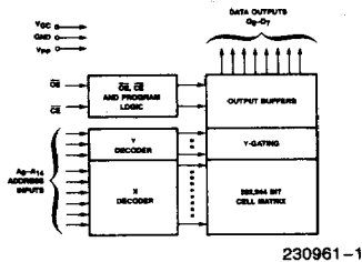
Figure 1. Block Diagram
