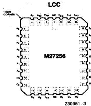
Figure 2. Pin Configurations
