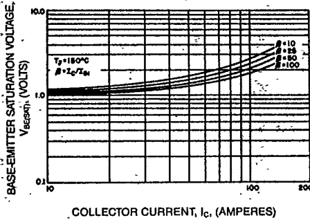
SATURATION VOLTAGE (TYPICAL)
