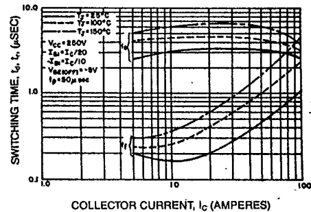
SWITCHING CHARACTERISTICS (TYPICAL)
