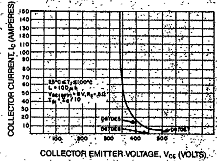
REVERSE BIAS SAFE OPERATING AREA (R.B.S.O.A.)
