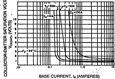
COLLECTOR-EMITTER SATURATION VOLTAGE (TYPICAL)
