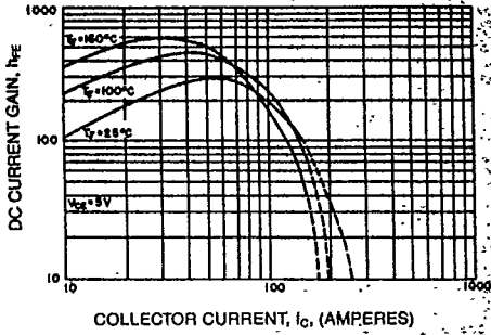
DC CURRENT GAIN (TYPICAL)
