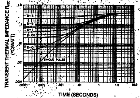
TRANSIENT THERMAL IMPEDANCE CHARACTERISTICS (TRANSISTOR)
