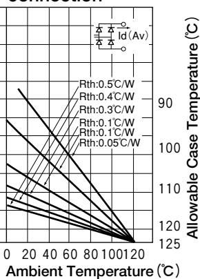
B2; Two Pulse Bridge connection
