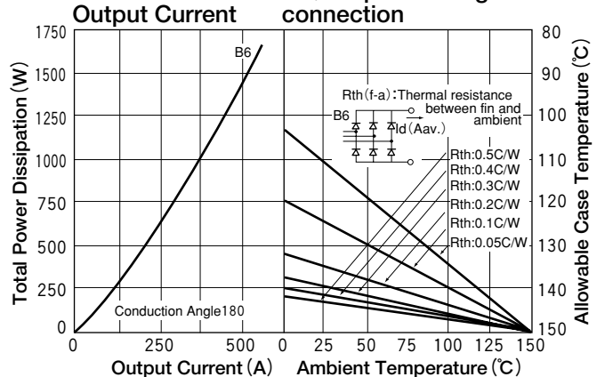
B6; Six pulse Bridge connection
