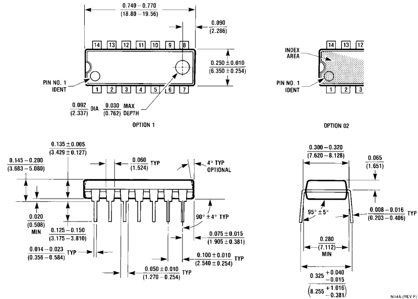
14-Lead Molded Dual-In-Line Package (N) Order Number DM7426N Package Number N14A
