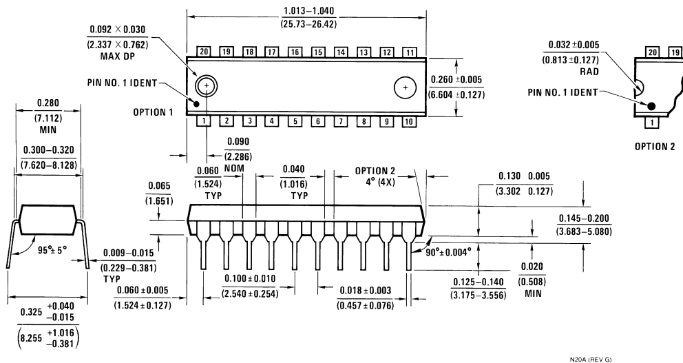
Molded Dual-In-Line Package (N) Order Number DM74ALS533N Package Number N20A
