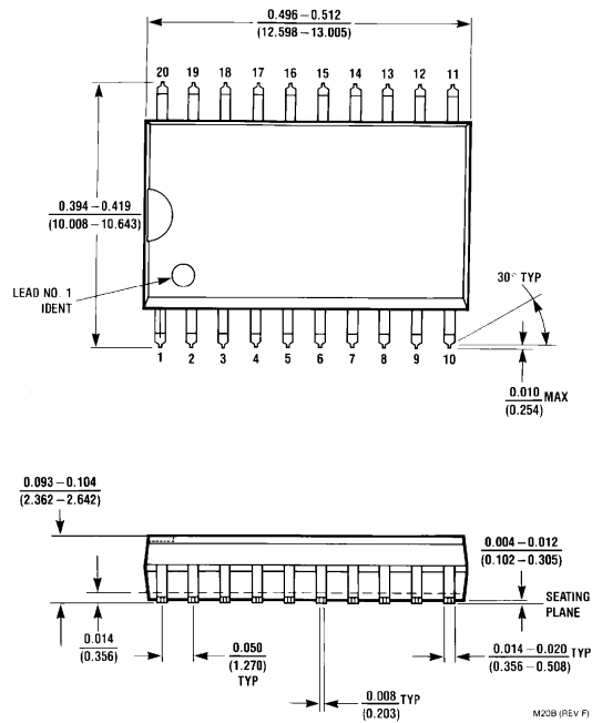
S.O. Package (M) Order Number DM74ALS533WM Package Number M20B
